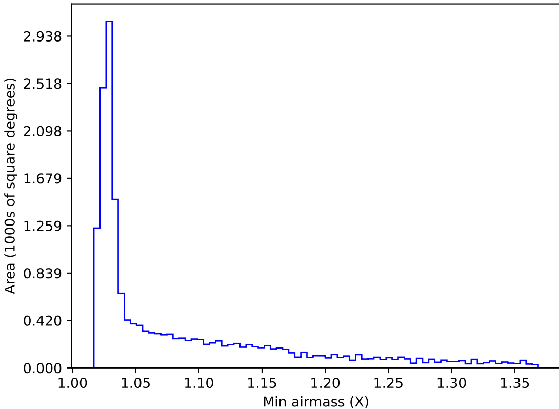
noroll_mjdp365_v3.4_10yrs WFD r band: Min airmass
