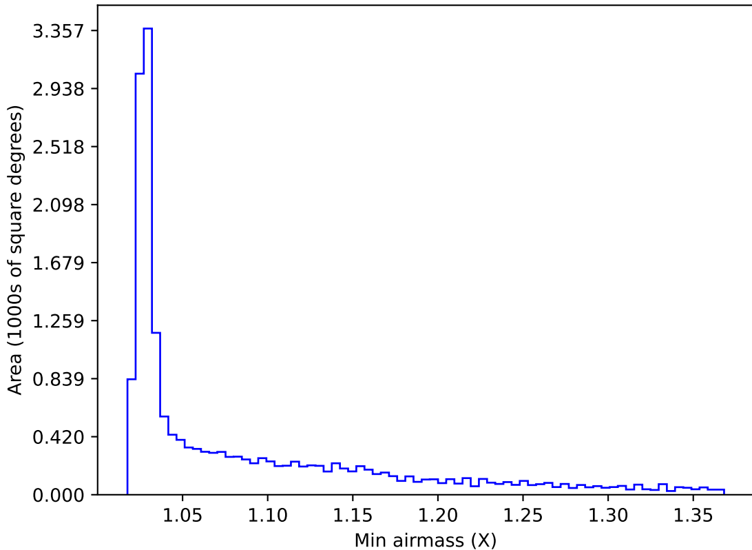
noroll_mjdp365_v3.4_10yrs WFD i band: Min airmass
