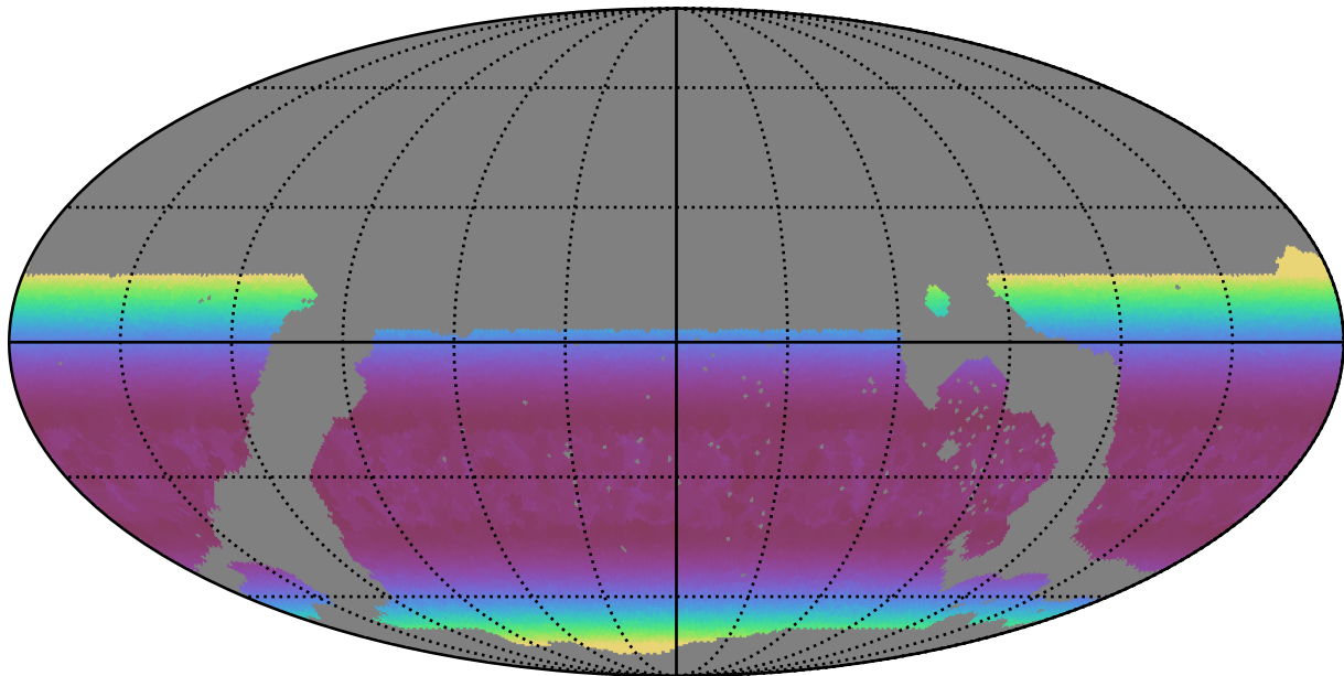
noroll_mjdp365_v3.4_10yrs WFD g band: Min airmass
