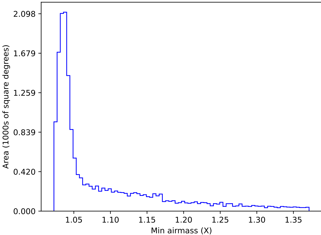
noroll_mjdp365_v3.4_10yrs WFD g band: Min airmass
