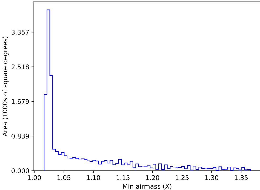
noroll_mjdp365_v3.4_10yrs WFD all bands: Min airmass
