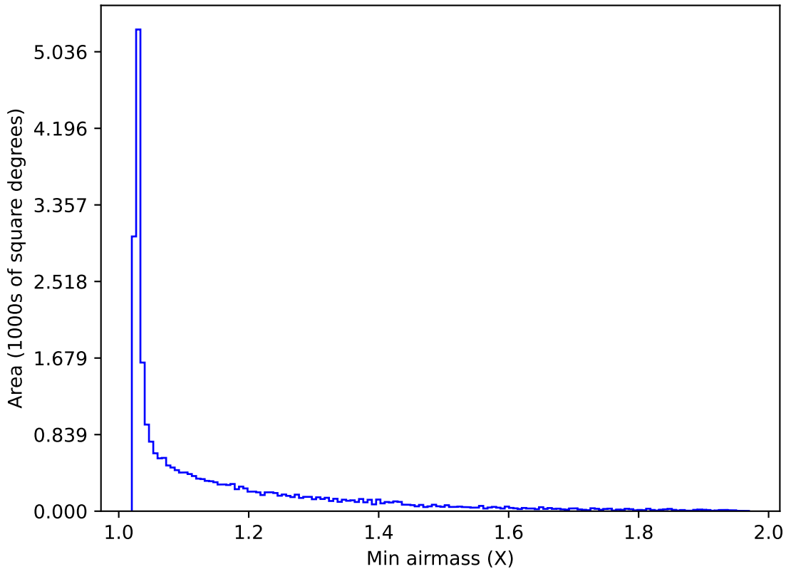
noroll_mjdp365_v3.4_10yrs All sky z band: Min airmass
