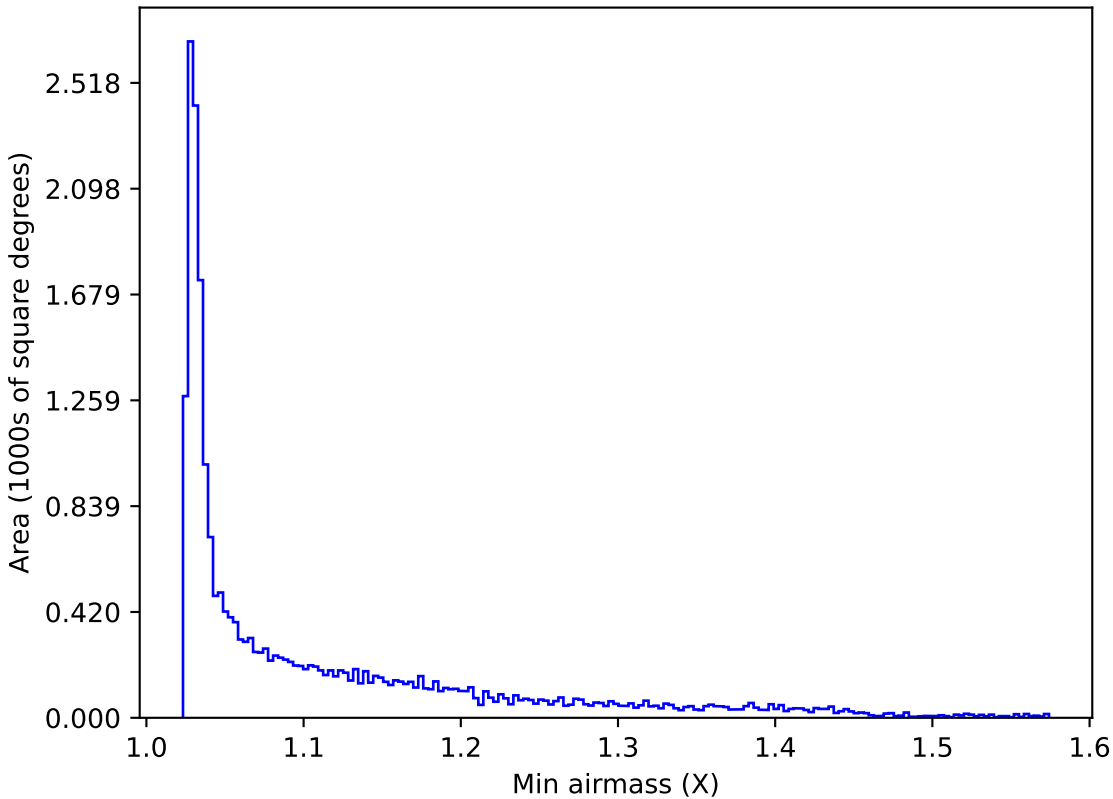
noroll_mjdp365_v3.4_10yrs All sky y band: Min airmass
