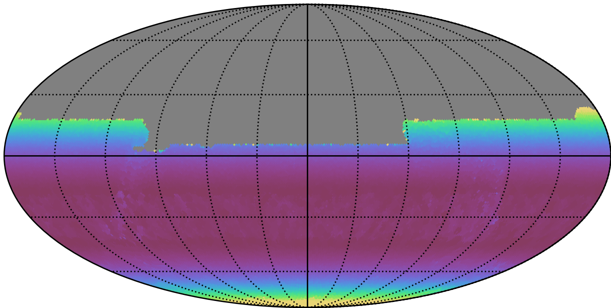
noroll_mjdp365_v3.4_10yrs All sky u band: Min airmass
