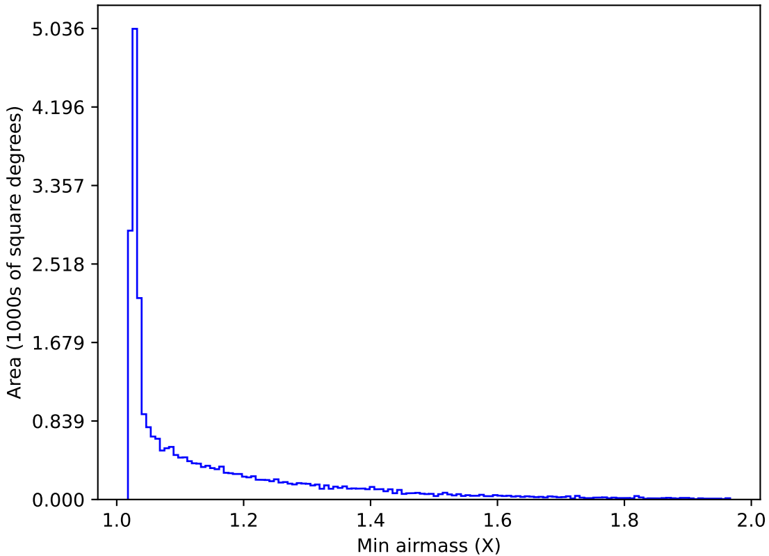
noroll_mjdp365_v3.4_10yrs All sky r band: Min airmass
