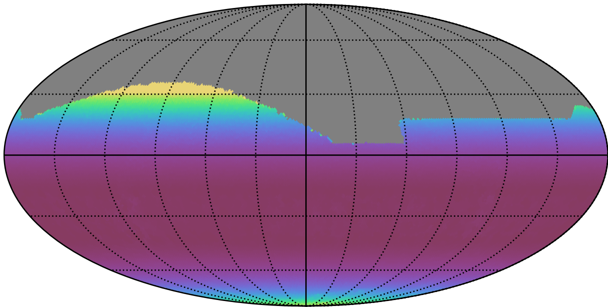
noroll_mjdp365_v3.4_10yrs All sky i band: Min airmass
