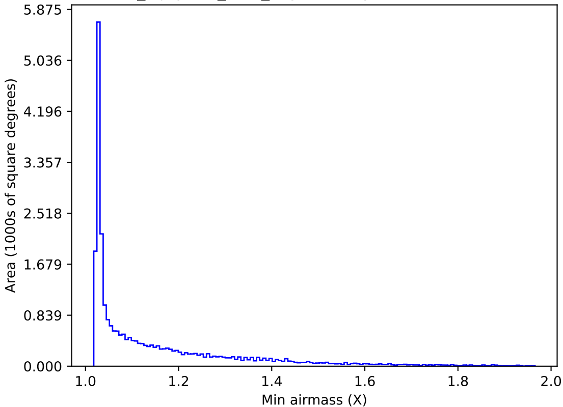
noroll_mjdp365_v3.4_10yrs All sky i band: Min airmass
