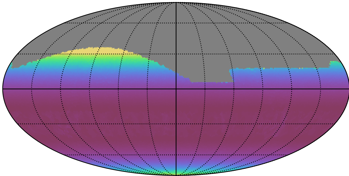
noroll_mjdp365_v3.4_10yrs All sky g band: Min airmass
