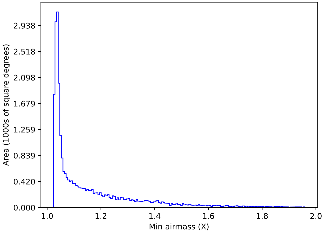
noroll_mjdp365_v3.4_10yrs All sky g band: Min airmass
