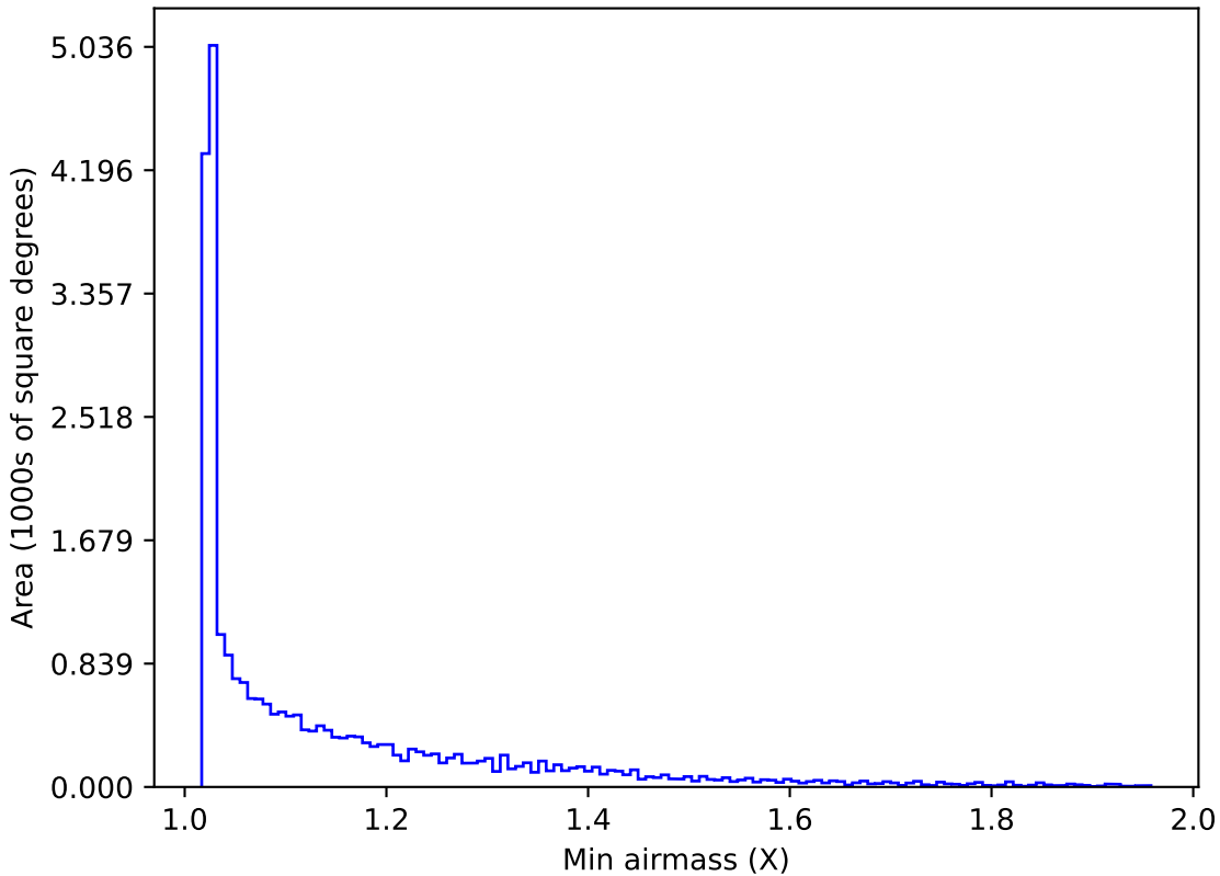
noroll_mjdp365_v3.4_10yrs All sky all bands: Min airmass
