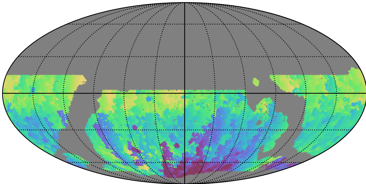
noroll_mjdp365_v3.4_10yrs WFD u band: Min HA
