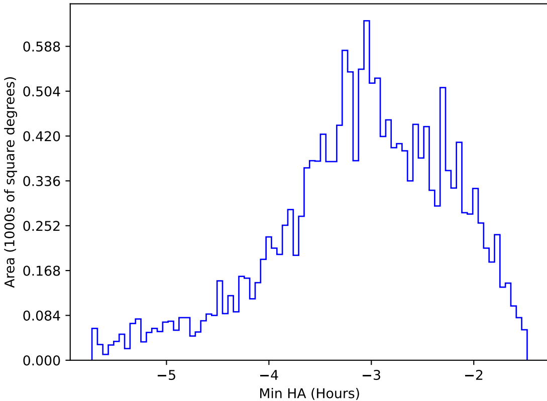
noroll_mjdp365_v3.4_10yrs WFD u band: Min HA
