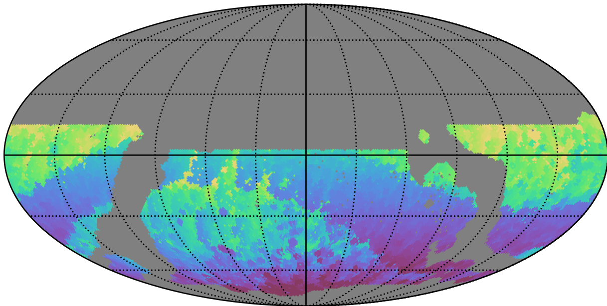
noroll_mjdp365_v3.4_10yrs WFD r band: Min HA
