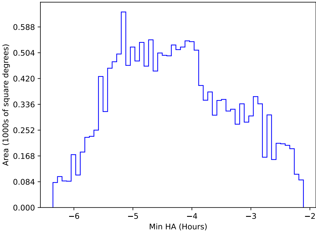
noroll_mjdp365_v3.4_10yrs WFD r band: Min HA
