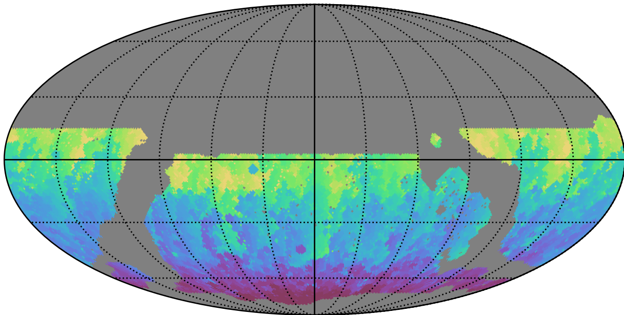
noroll_mjdp365_v3.4_10yrs WFD g band: Min HA
