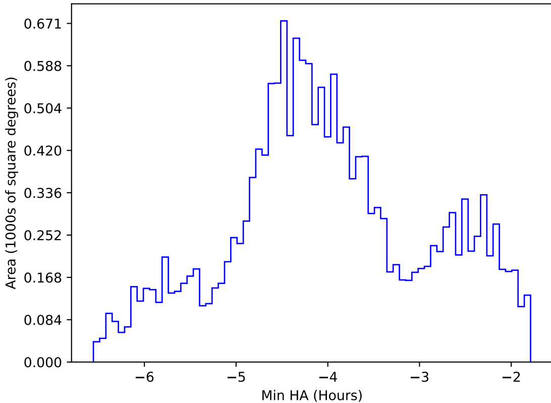
noroll_mjdp365_v3.4_10yrs WFD g band: Min HA
