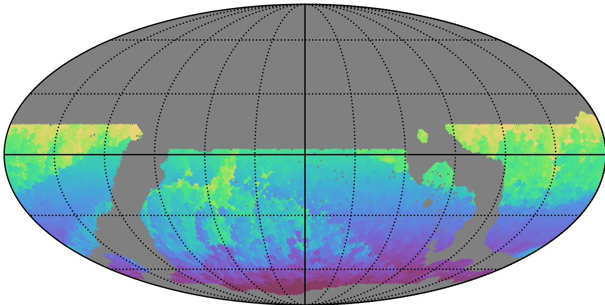
noroll_mjdp365_v3.4_10yrs WFD all bands: Min HA
