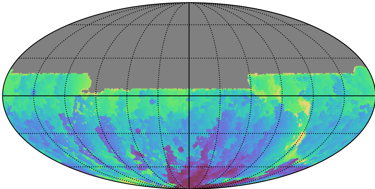
noroll_mjdp365_v3.4_10yrs All sky u band: Min HA
