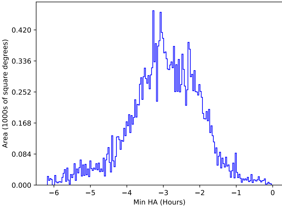
noroll_mjdp365_v3.4_10yrs All sky u band: Min HA
