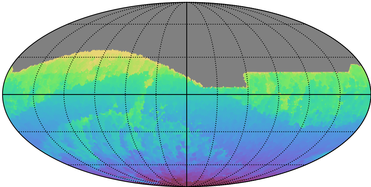
noroll_mjdp365_v3.4_10yrs All sky all bands: Min HA
