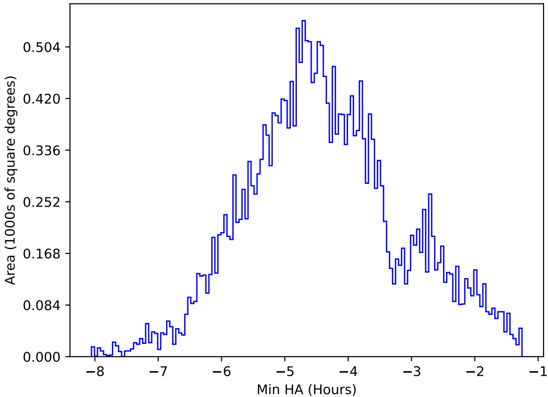
noroll_mjdp365_v3.4_10yrs All sky all bands: Min HA
