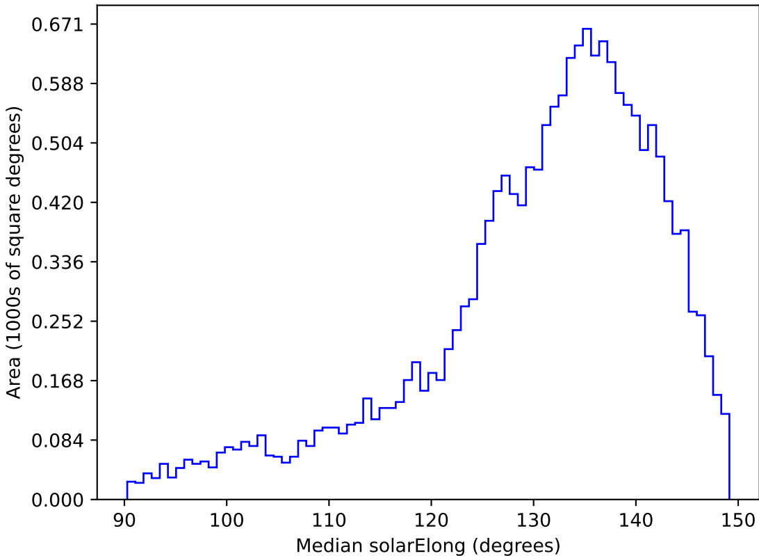
noroll_mjdp365_v3.4_10yrs WFD y band: Median solarElong
