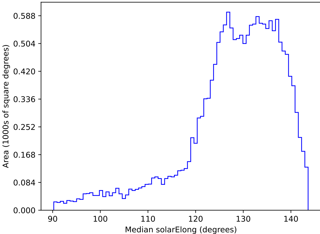
noroll_mjdp365_v3.4_10yrs WFD i band: Median solarElong
