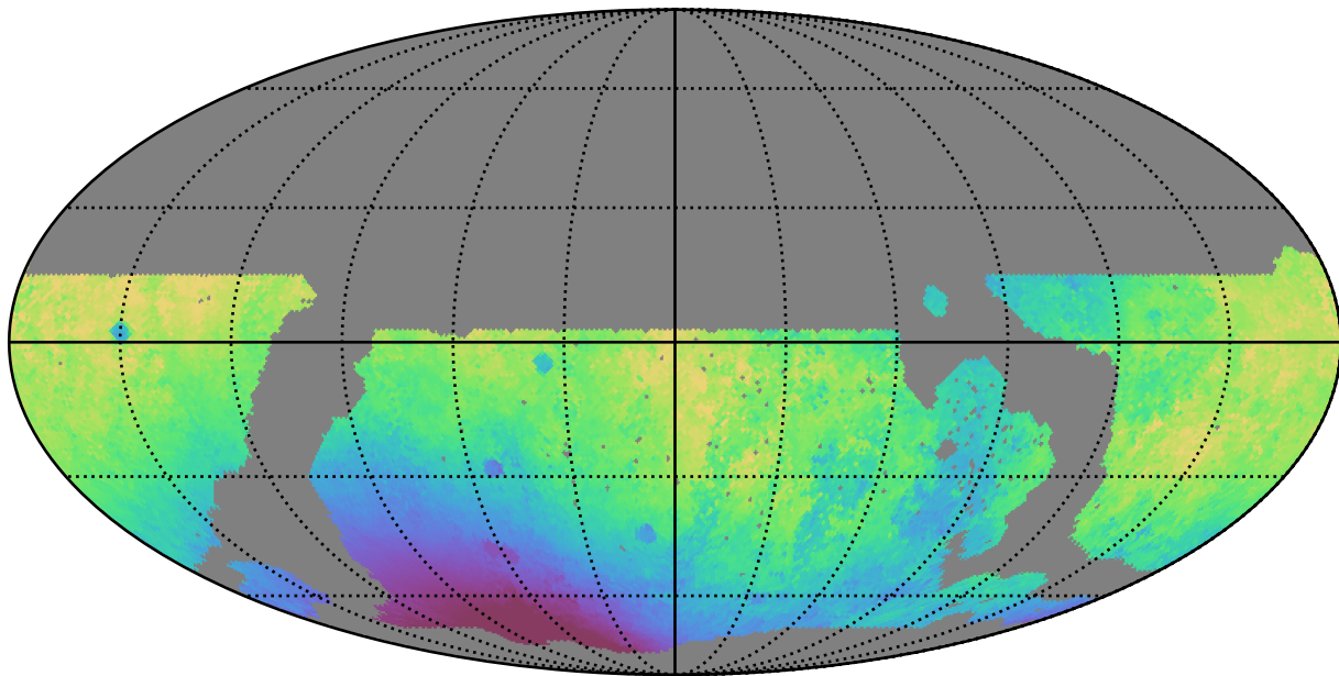
noroll_mjdp365_v3.4_10yrs WFD g band: Median solarElong
