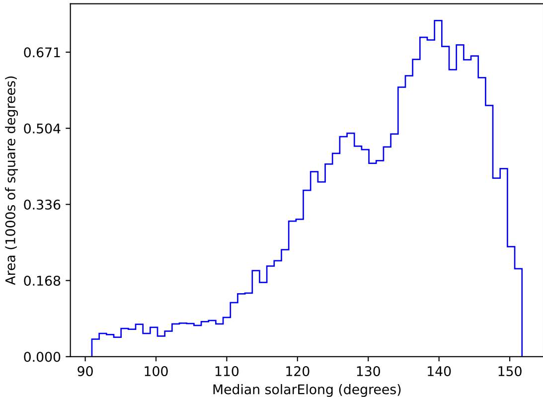
noroll_mjdp365_v3.4_10yrs WFD g band: Median solarElong
