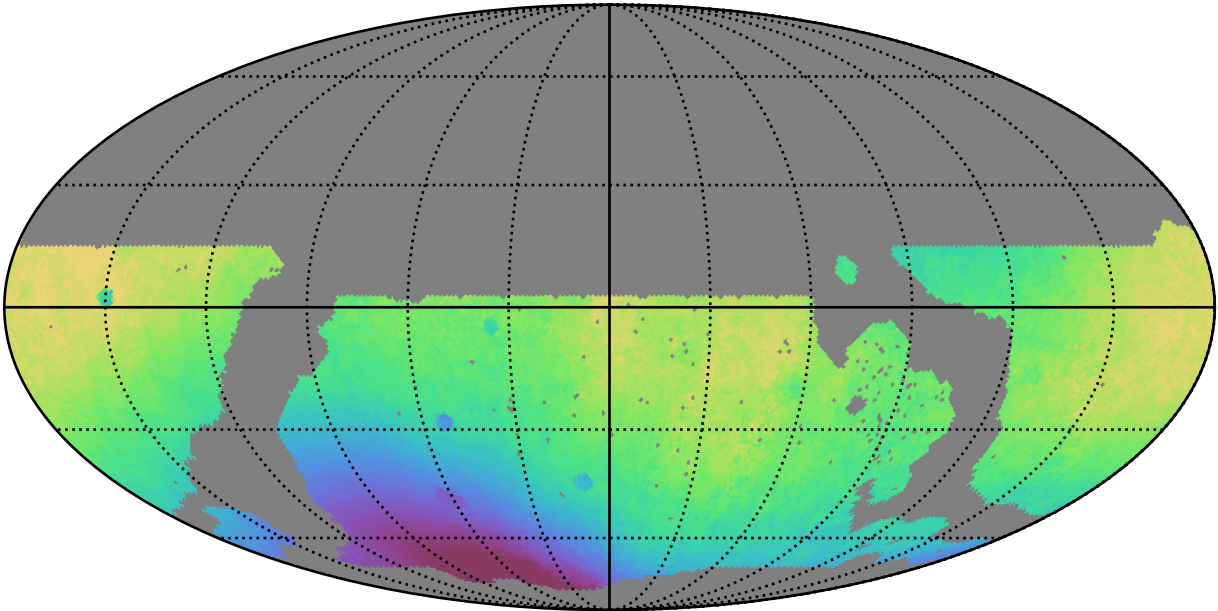
noroll_mjdp365_v3.4_10yrs WFD all bands: Median solarElong
