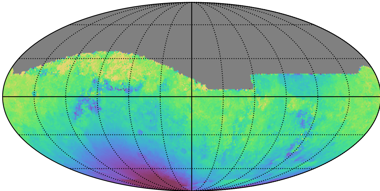
noroll_mjdp365_v3.4_10yrs All sky z band: Median solarElong
