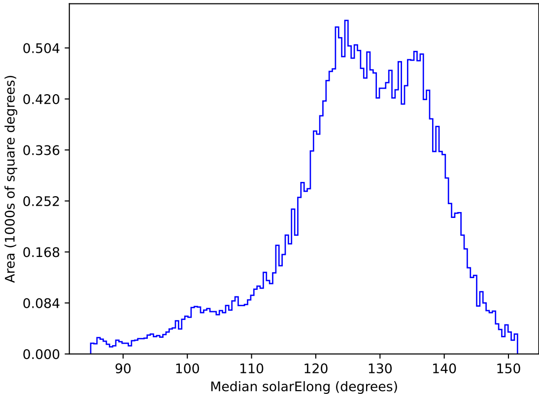
noroll_mjdp365_v3.4_10yrs All sky z band: Median solarElong
