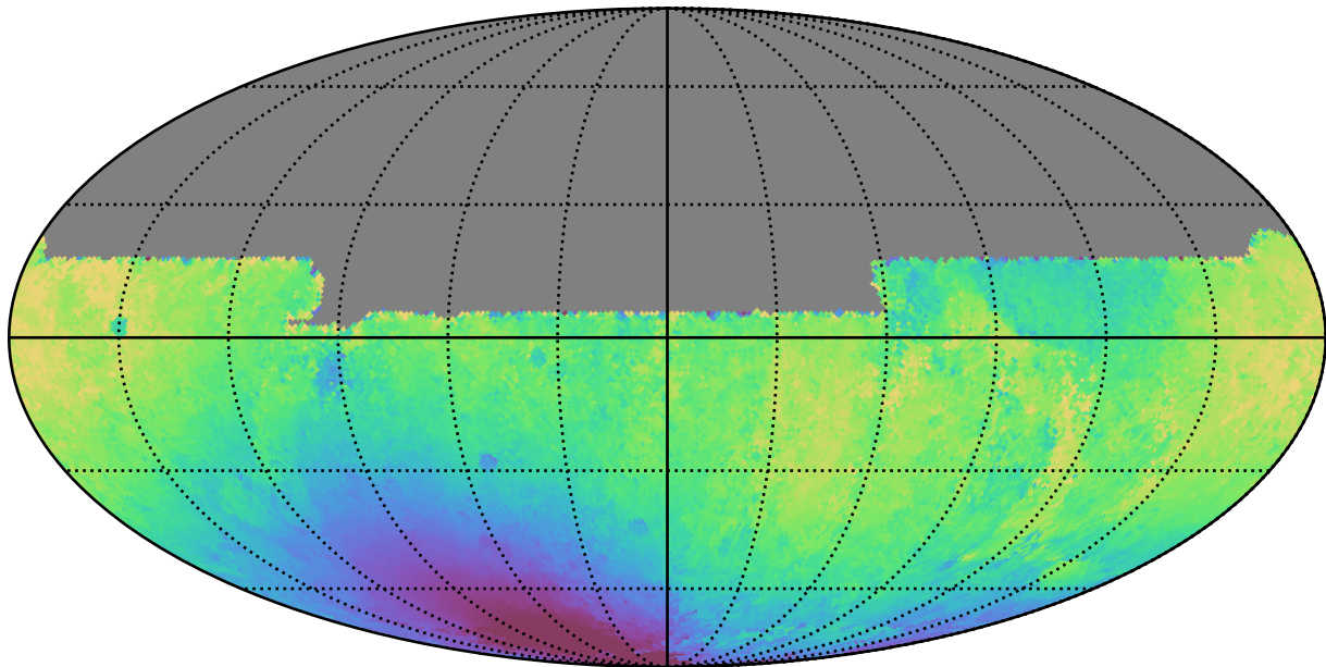
noroll_mjdp365_v3.4_10yrs All sky y band: Median solarElong
