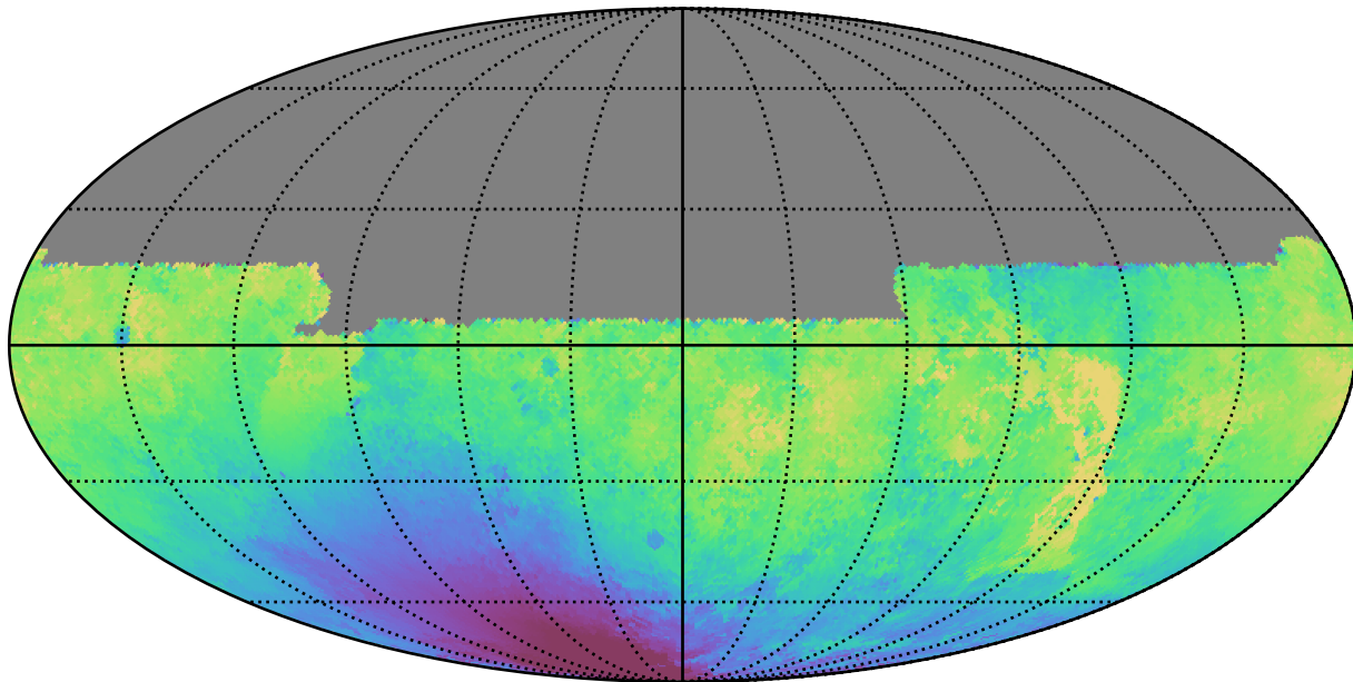
noroll_mjdp365_v3.4_10yrs All sky u band: Median solarElong
