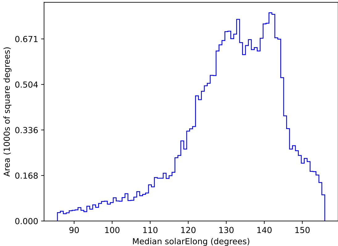
noroll_mjdp365_v3.4_10yrs All sky r band: Median solarElong
