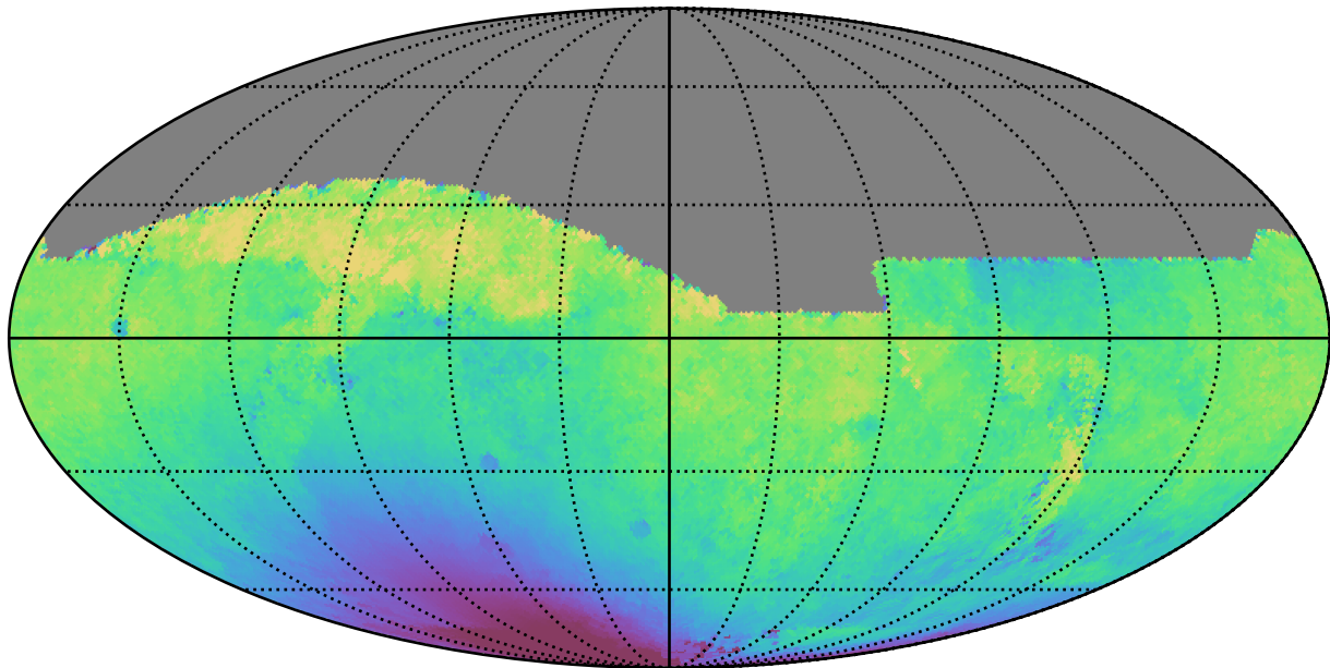
noroll_mjdp365_v3.4_10yrs All sky i band: Median solarElong
