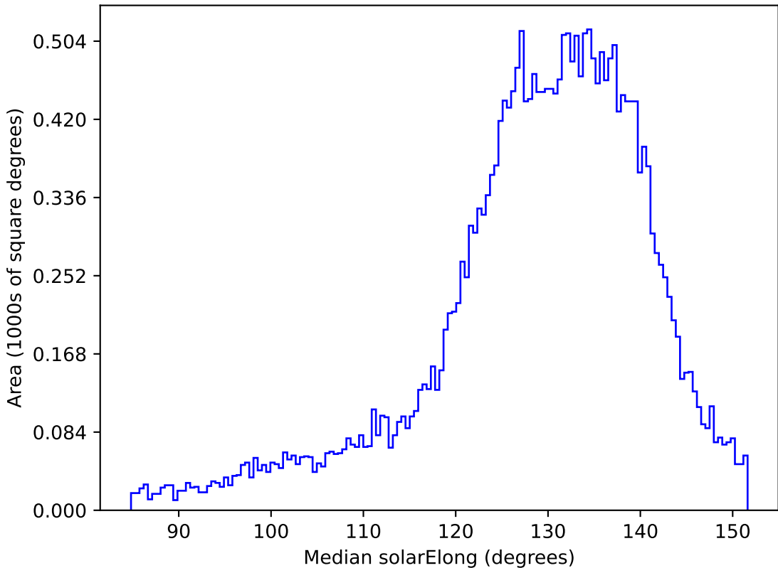
noroll_mjdp365_v3.4_10yrs All sky i band: Median solarElong
