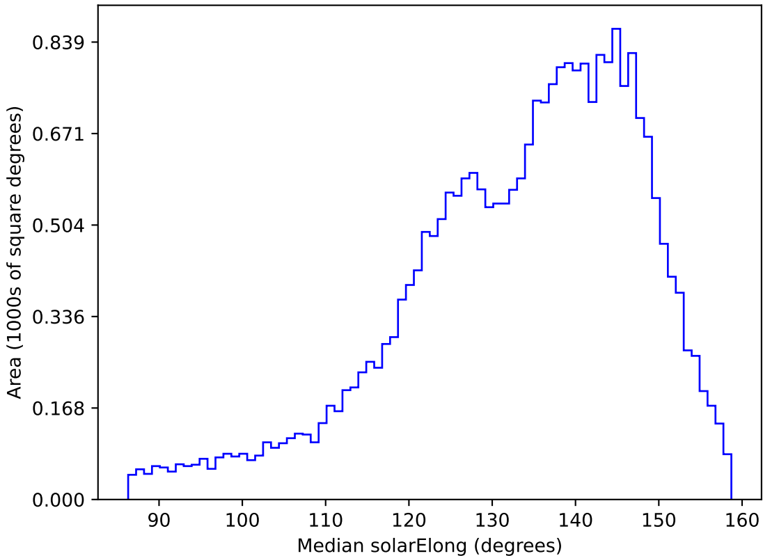
noroll_mjdp365_v3.4_10yrs All sky g band: Median solarElong
