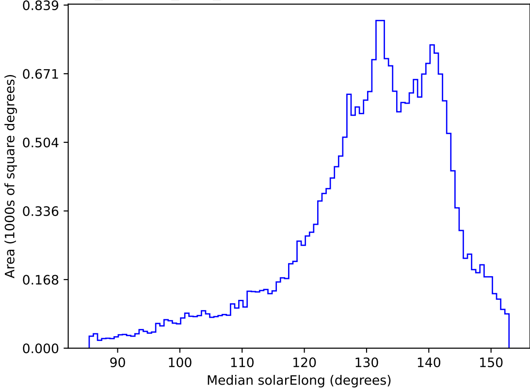
noroll_mjdp365_v3.4_10yrs All sky all bands: Median solarElong
