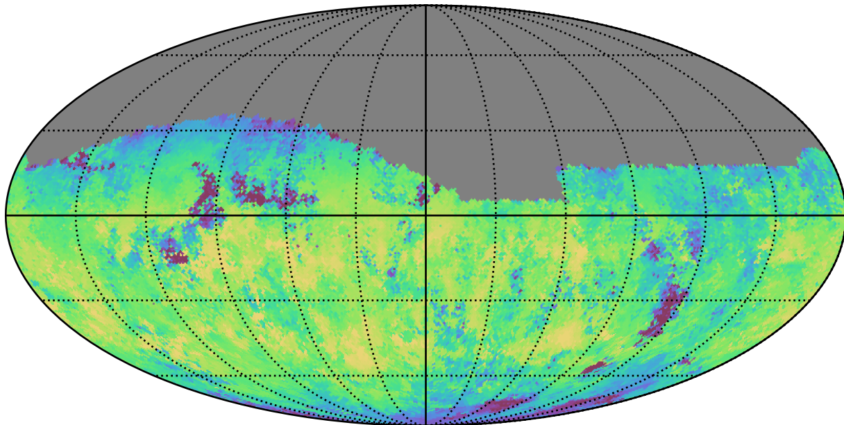
noroll_mjdp365_v3.4_10yrs Yr 1 z band: Median skyBrightness
