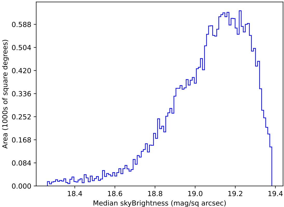
noroll_mjdp365_v3.4_10yrs Yr 1 z band: Median skyBrightness
