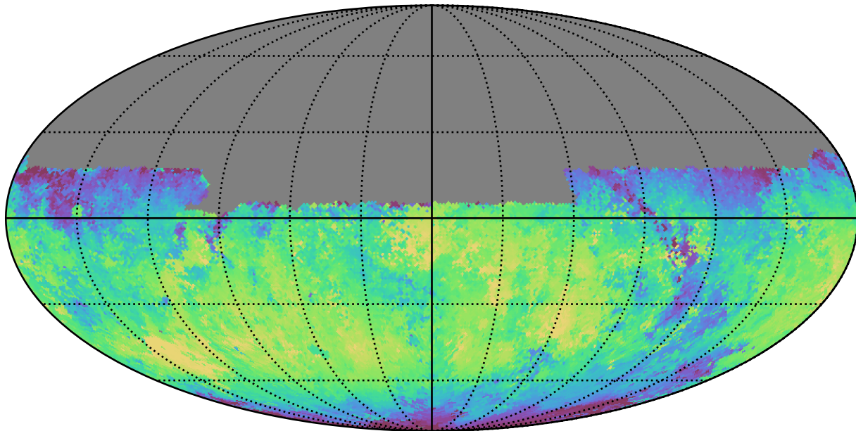
noroll_mjdp365_v3.4_10yrs Yr 1 y band: Median skyBrightness
