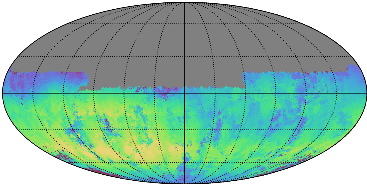
noroll_mjdp365_v3.4_10yrs Yr 1 u band: Median skyBrightness
