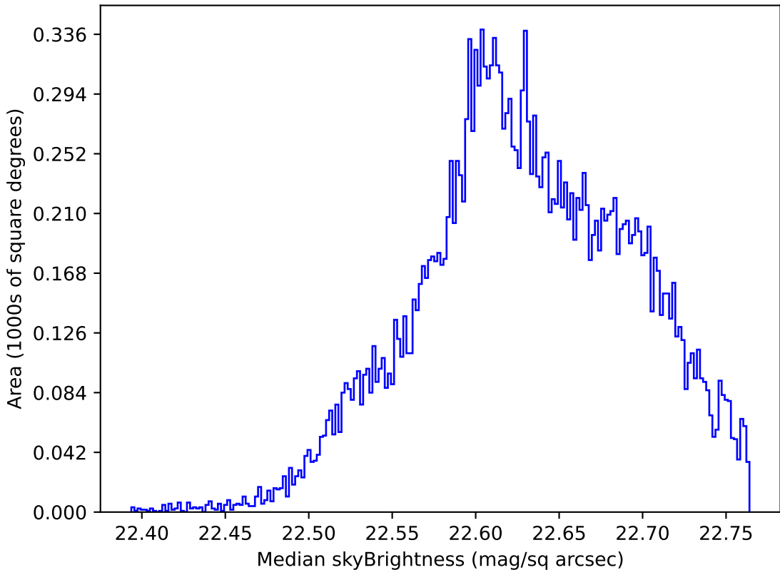
noroll_mjdp365_v3.4_10yrs Yr 1 u band: Median skyBrightness
