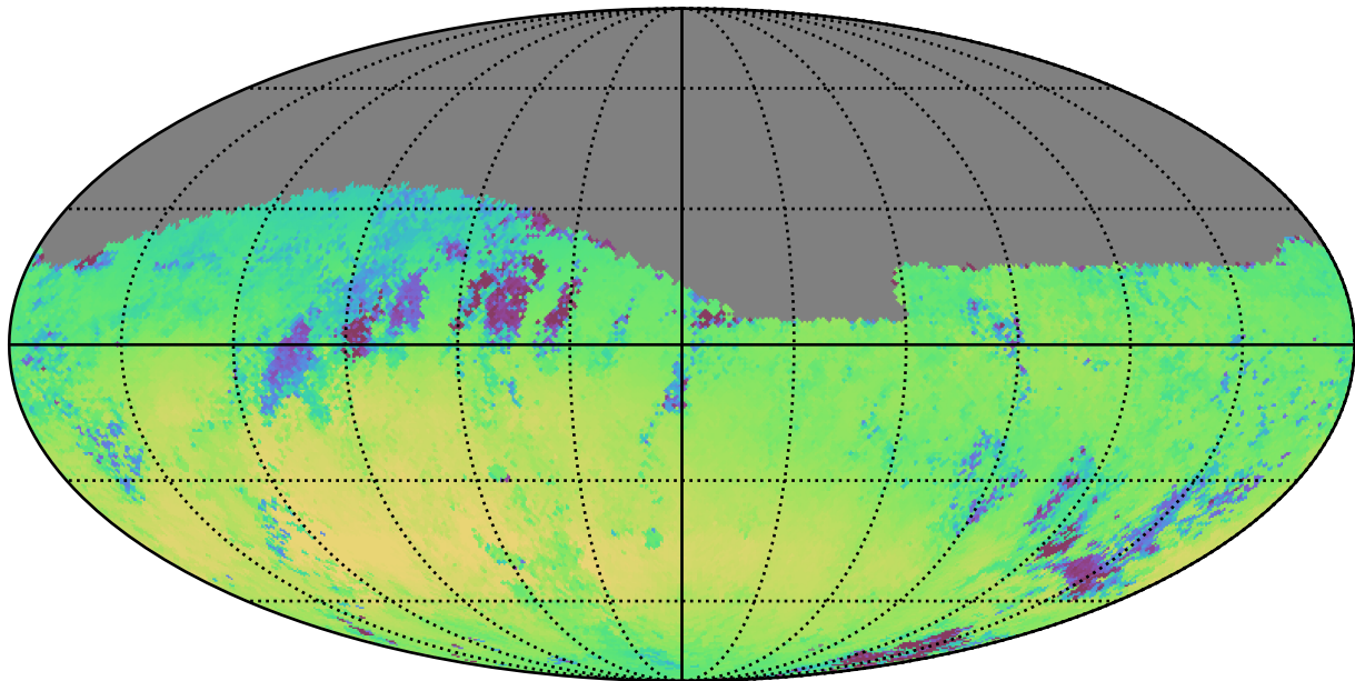
noroll_mjdp365_v3.4_10yrs Yr 1 r band: Median skyBrightness
