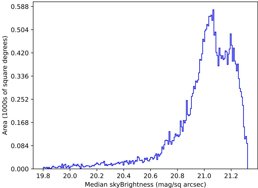
noroll_mjdp365_v3.4_10yrs Yr 1 r band: Median skyBrightness
