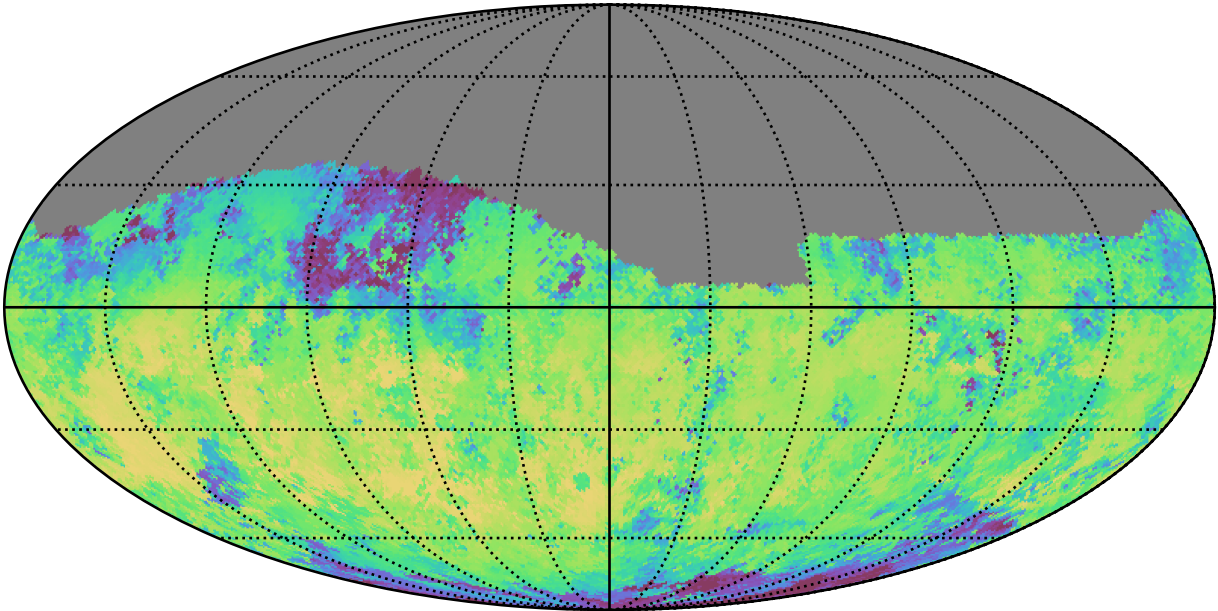
noroll_mjdp365_v3.4_10yrs Yr 1 i band: Median skyBrightness
