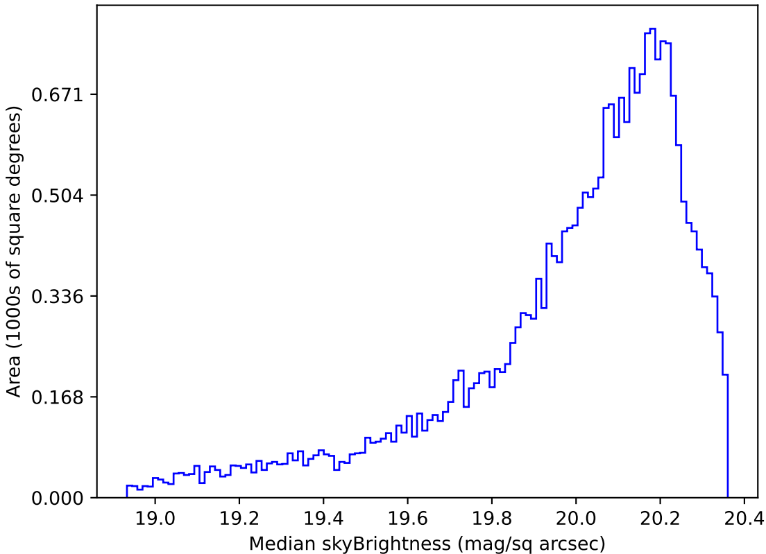
noroll_mjdp365_v3.4_10yrs Yr 1 i band: Median skyBrightness
