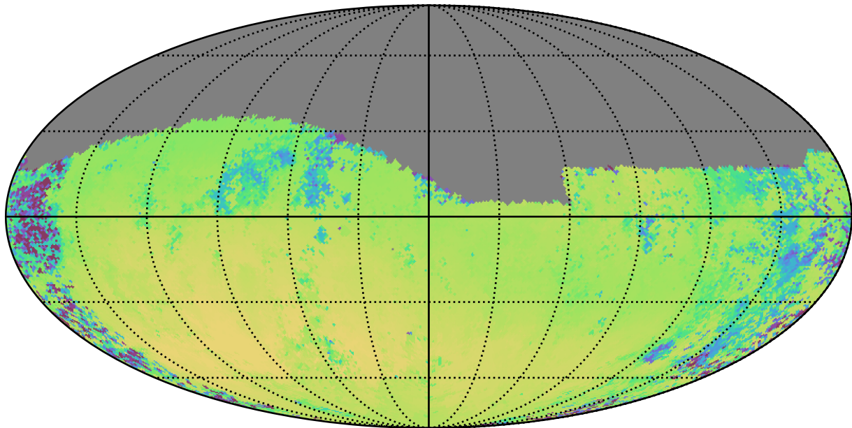
noroll_mjdp365_v3.4_10yrs Yr 1 g band: Median skyBrightness
