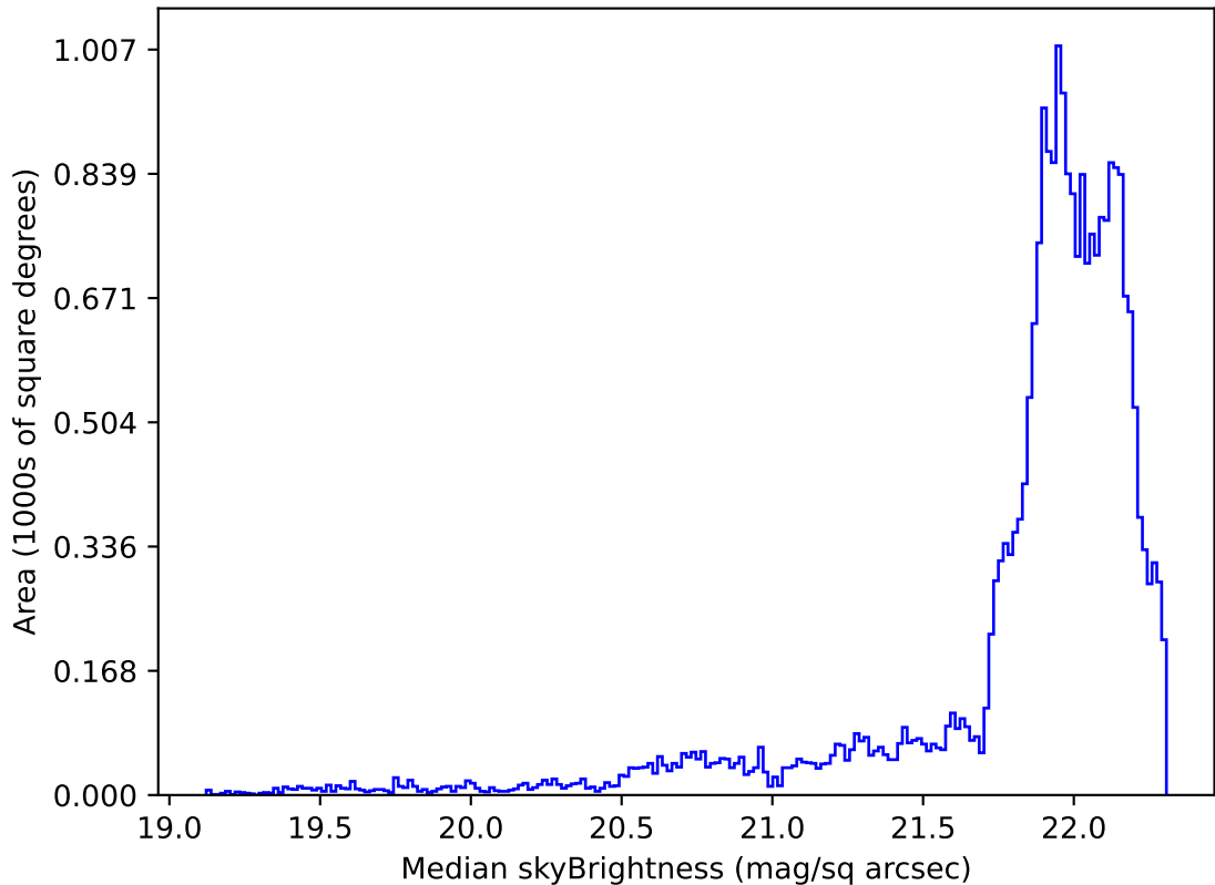
noroll_mjdp365_v3.4_10yrs Yr 1 g band: Median skyBrightness
